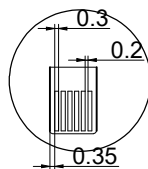
DETAIL "A" 4:1
